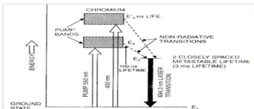
Energy levels of chromium ions in Ruby laser
